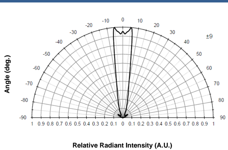
Radiation Characteristics
