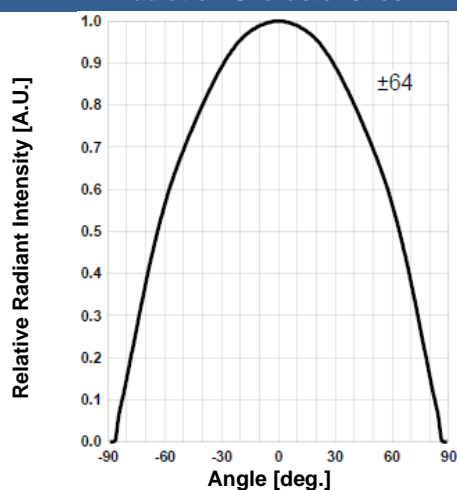
Radiation Characteristics
