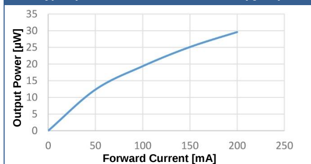
Typ. Optical Power Characteristics (QCW)
