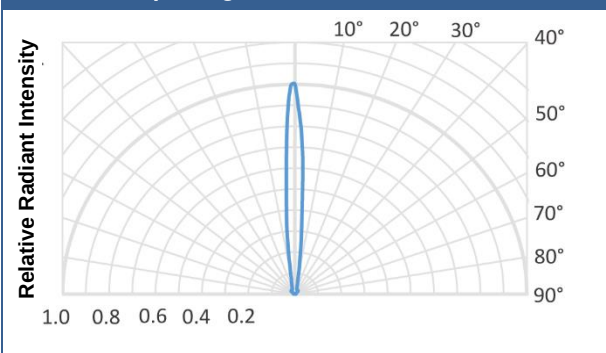
TO-18 package with Parabolic Reflector
