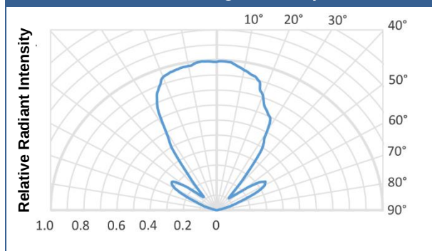
TO-18 Package With Cap
