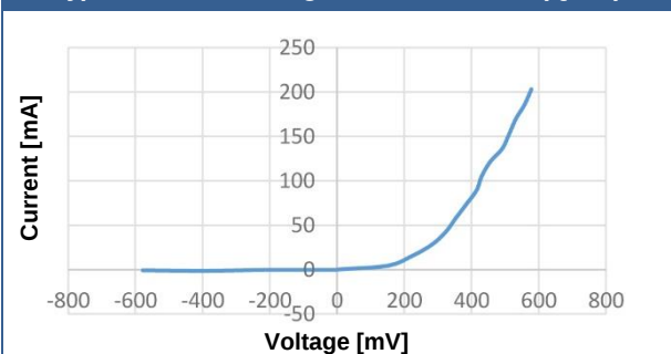
Typ. Current – Voltage Characteristics (QCW)
