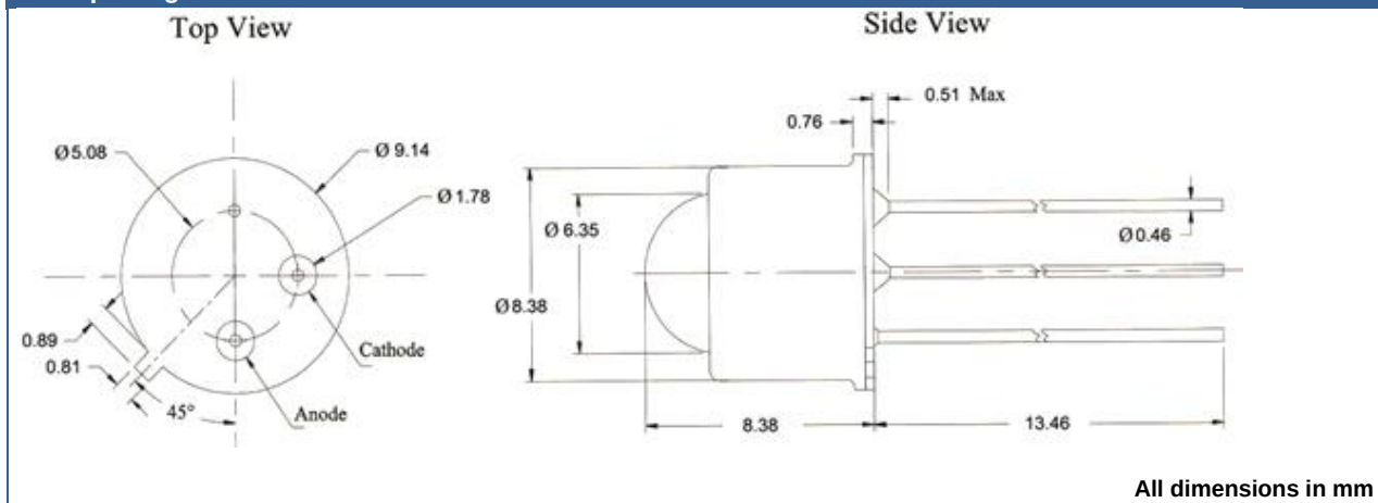
TO39 package
